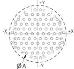
73 contacts size 23
