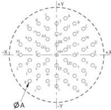
53 contacts size 20
