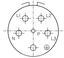
Layout example 17-V6 / 17-E6
