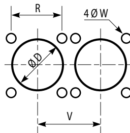
LJT 00 Square flange receptacle Front panel mounting
