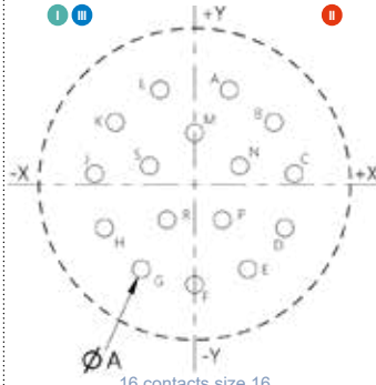
16 contacts size 16
