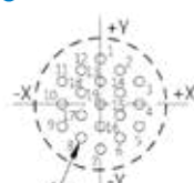
19 contacts size 23
