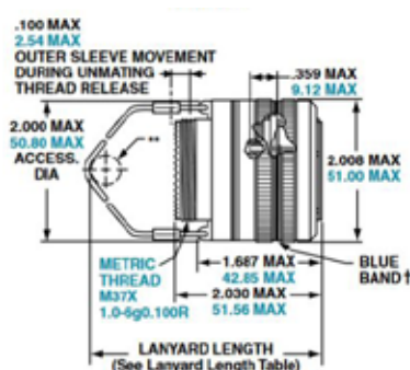
Type 6 MILITARY. D38999/31**6
