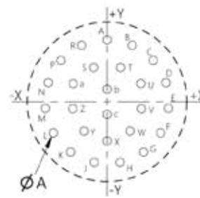
26 contacts size 20
