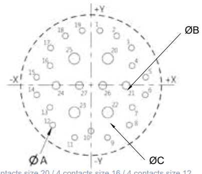
19 contacts size 20 / 4 contacts size 16 / 4 contacts size 12
