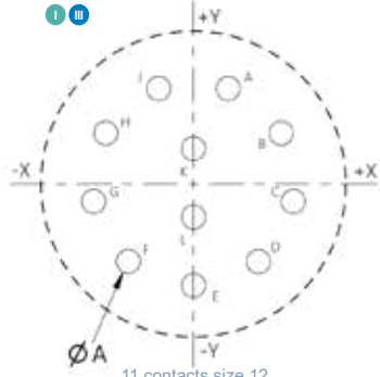
11 contacts size 12
