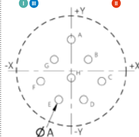
8 contacts size 16
