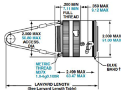
Type 1 (longer shell) MILITARY. D38999/31**1
