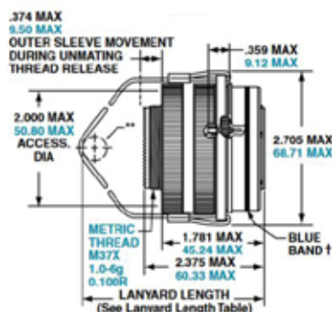
Type 2 MILITARY. D38999/31**2
