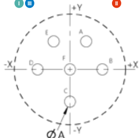
6 contacts size 12
