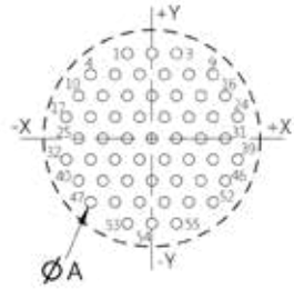
55 contacts size 23
