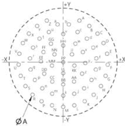
61 contacts size 20
