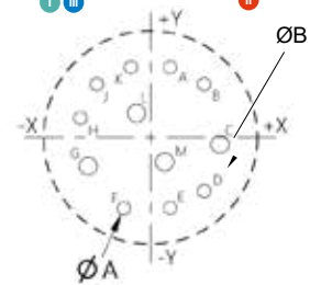
8 contacts size 20 4 contacts size 16
