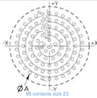
88 contacts size 23
