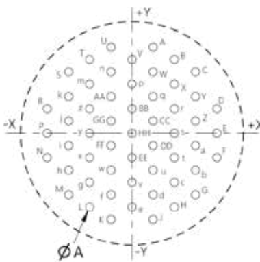
55 contacts size 20
